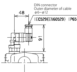
E,D: Electric contact type indicator 3501-□□-□□-□□-ED□
